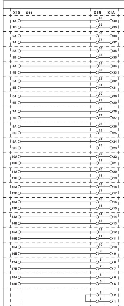
Circuit diagram
