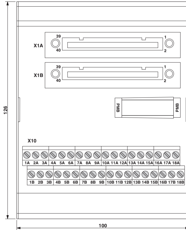
Dimensional drawing
