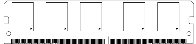
Figure 1: 288-Pin VLP MiniUDIMM (MO-314, R/C ZZ)
