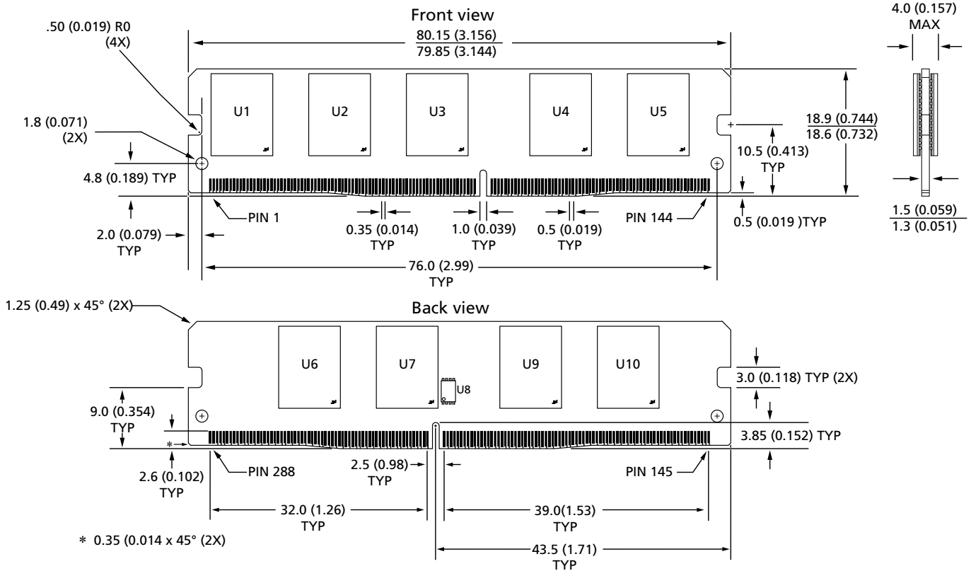
Figure 3: 288-Pin DDR4 VLP MiniUDIMM
