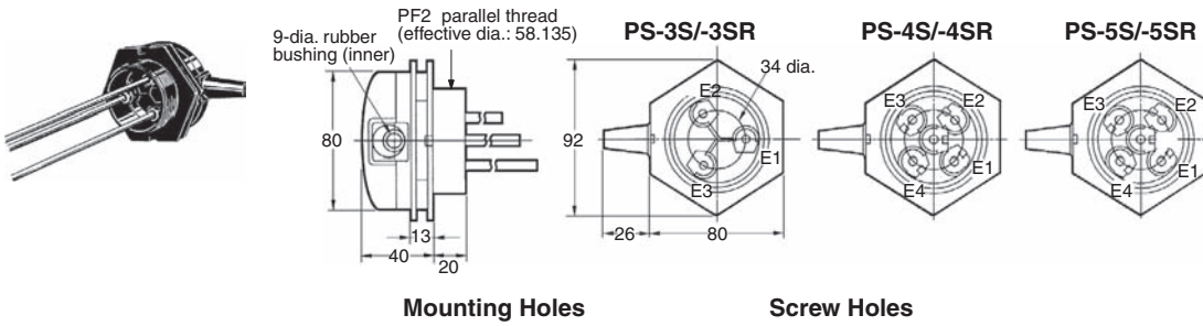
Mounting Holes
