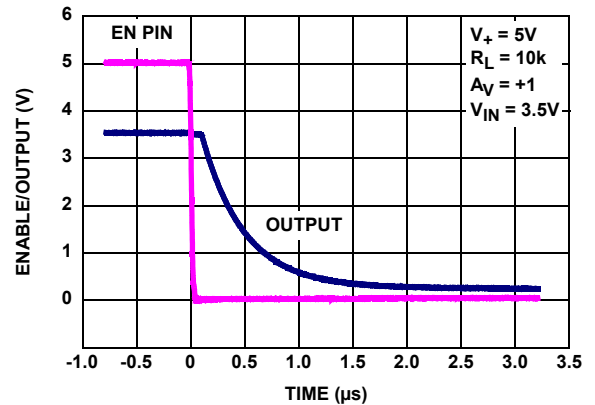
FIGURE 10. DISABLE TO OUTPUT DELAY TIME
