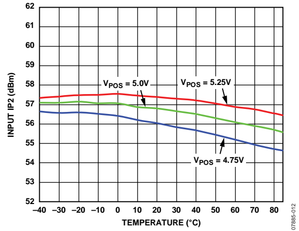
Figure 12. Input IP2 vs. Temperature
