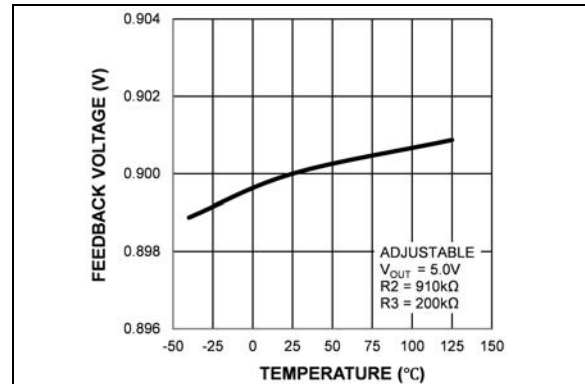
FIGURE 2-6: Feedback Voltage vs. Temperature.
